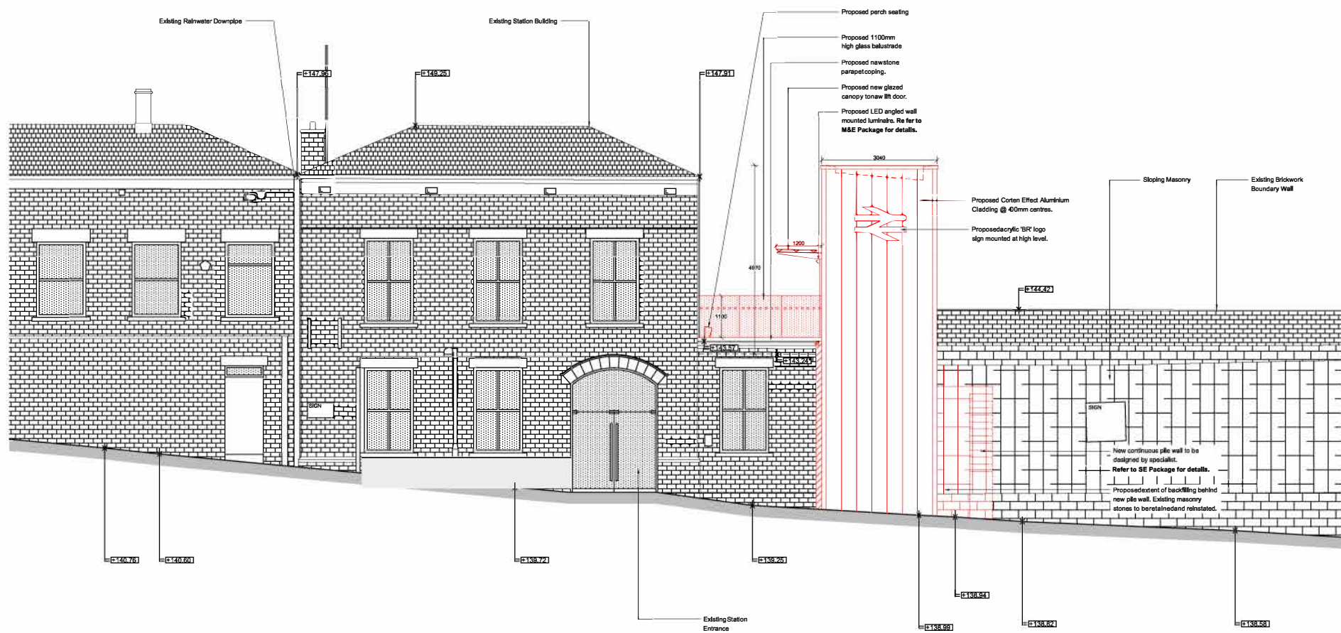
Proposed Section EE Scale 1 : 50 @ A1
