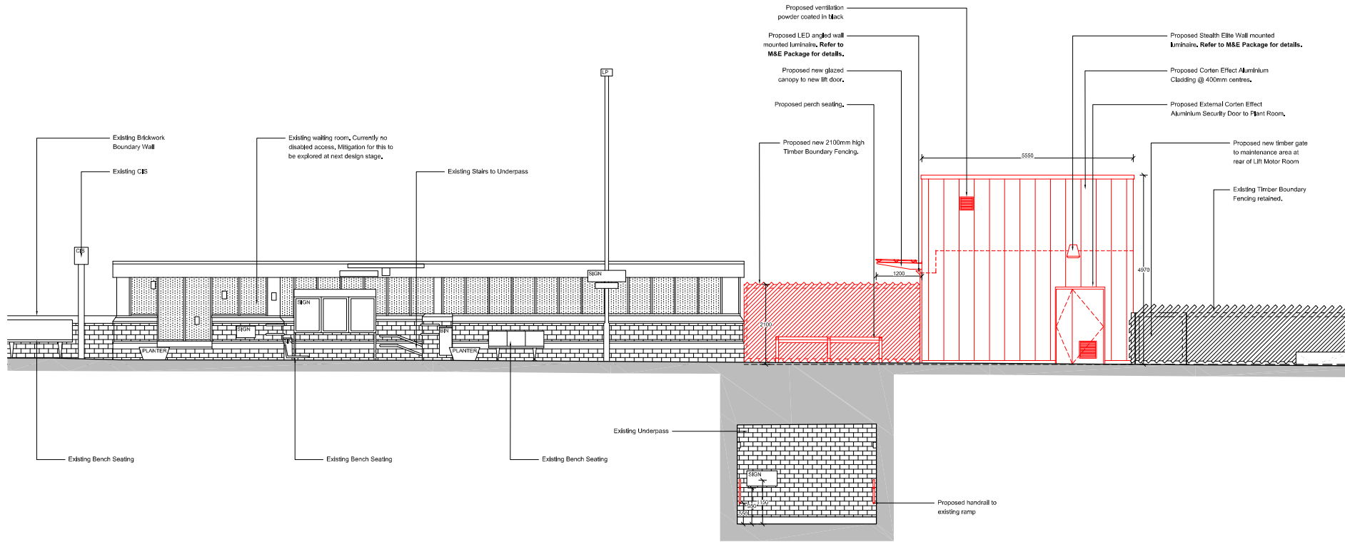
Proposed Section AA Scale 1 : 50 @ A1
